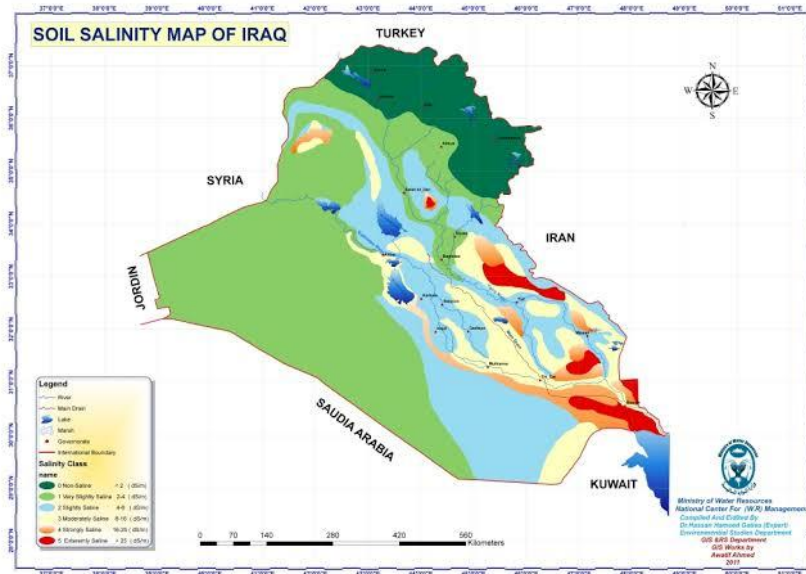
Figure 9. Subsurface salinity in Iraq [69]
